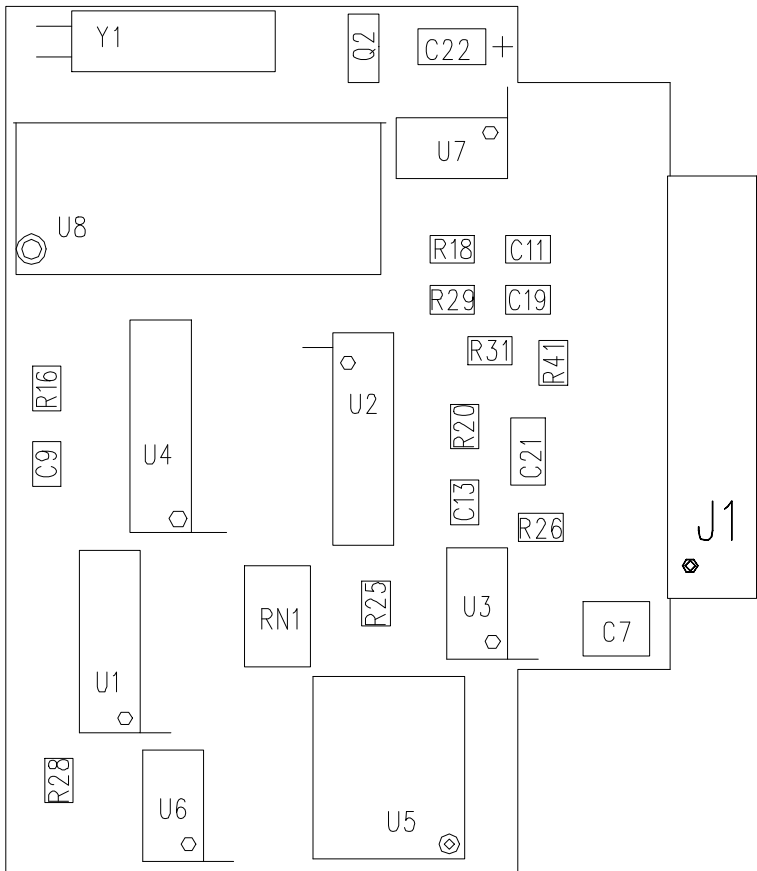
TOP SIDE VIEW
