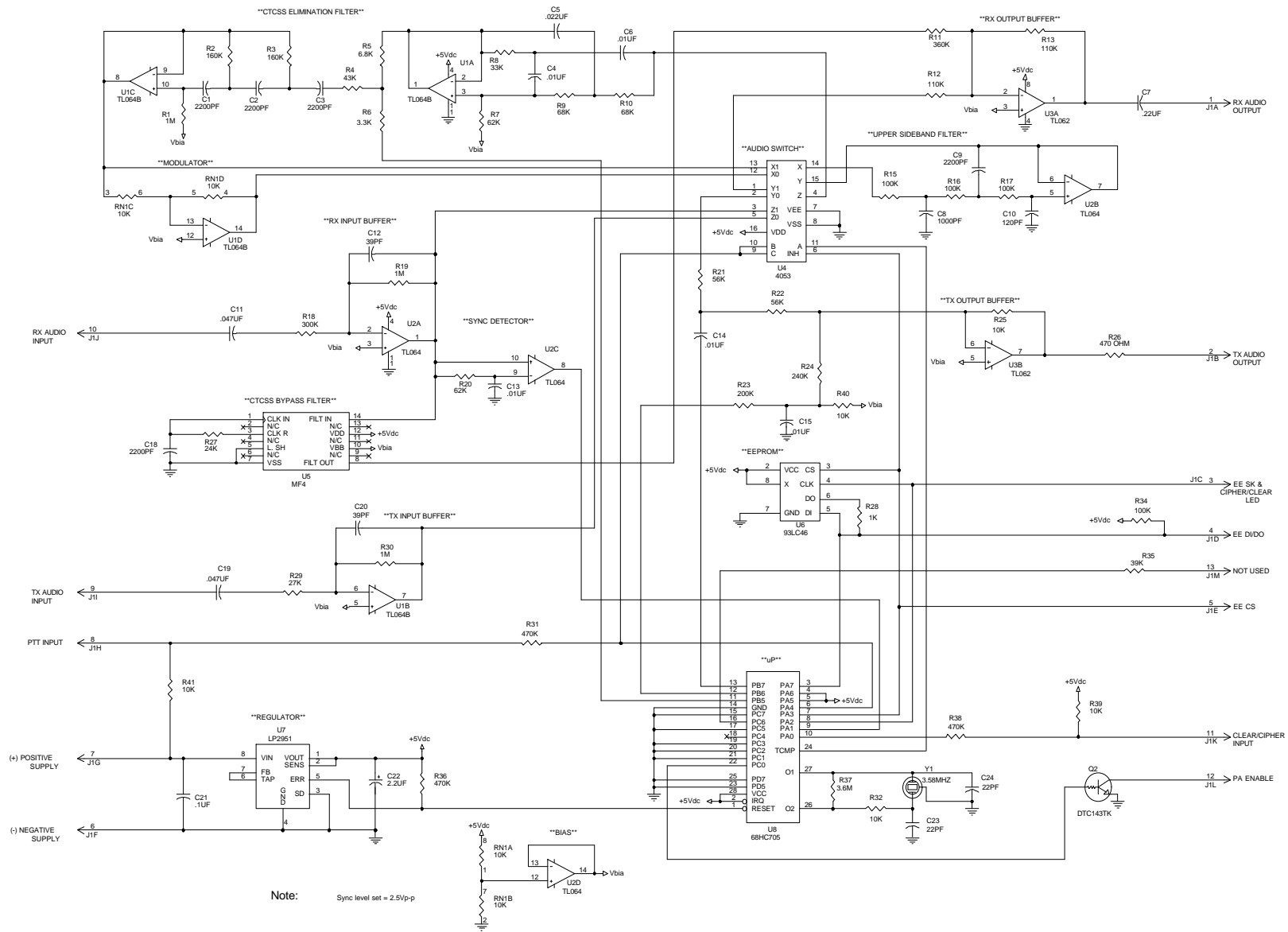
Figure 8 - ST-25AMC/AMT Schematic Diagram
