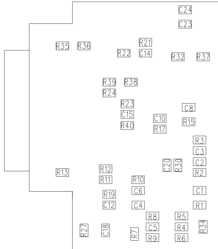
BOTTOM SIDE VIEW
